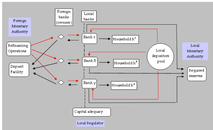
Fig. 1 Model Architecture
